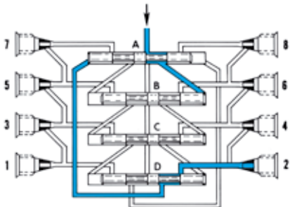
Lincoln systems with PTP divider block
